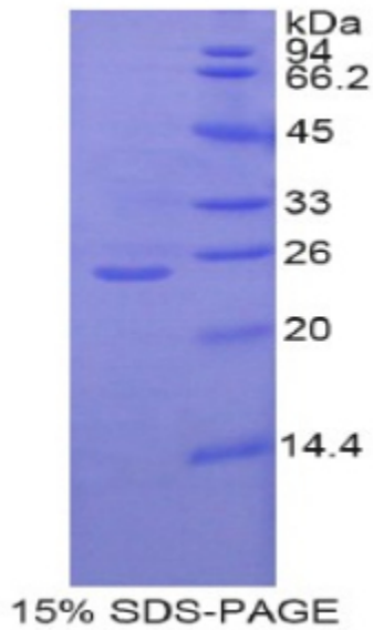
SDS-PAGE Image
