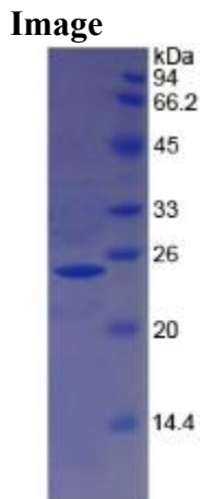
Figure. SDS-PAGE
