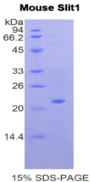
SDS-PAGE Image
