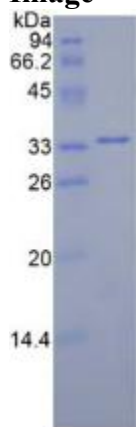
SDS-PAGE Image
