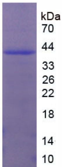
Figure. SDS-PAGE
