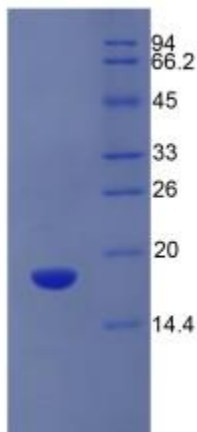
SDS-PAGE Image
