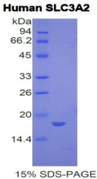
SDS-PAGE Image
