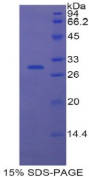
SDS-PAGE Image
