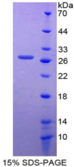
Figure. SDS-PAGE
