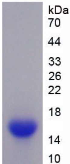
Figure. SDS-PAGE
