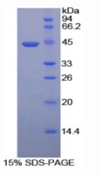
SDS-PAGE Image
