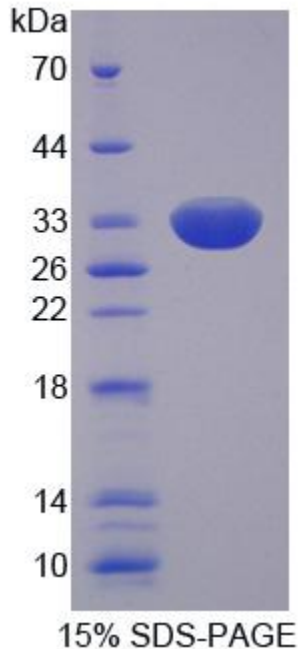
Figure. SDS-PAGE
