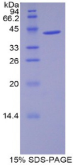
SDS-PAGE Image
