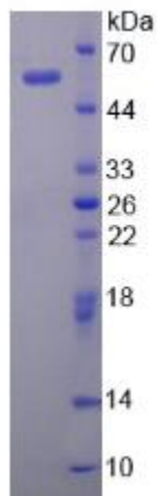
Figure. SDS-PAGE
