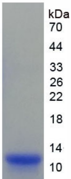
Figure. SDS-PAGE
