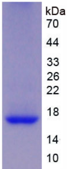
Figure. SDS-PAGE
