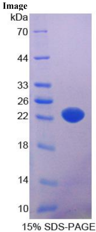
SDS-PAGE Image
