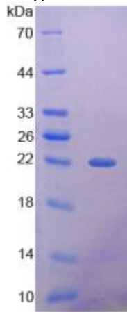
SDS-PAGE Image
