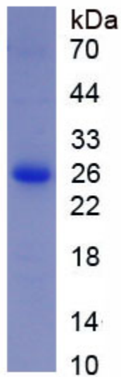
Figure. SDS-PAGE
