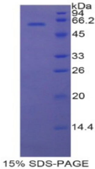
SDS-PAGE Image
