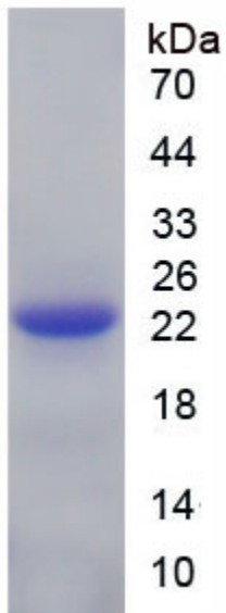
Figure. SDS-PAGE
