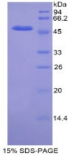
SDS-PAGE Image
