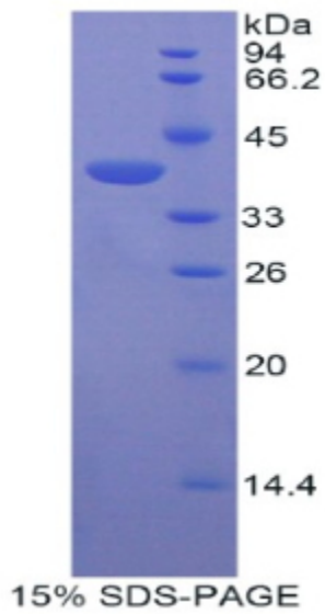
SDS-PAGE Image
