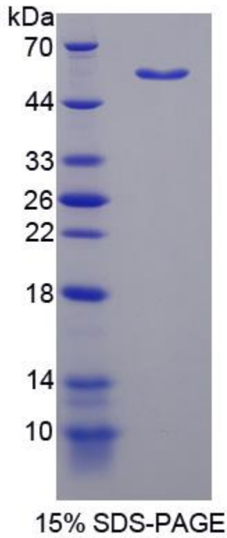
SDS-PAGE Image
