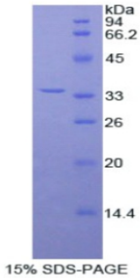
SDS-PAGE Image
