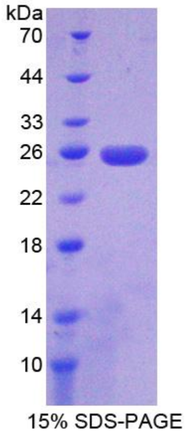
SDS-PAGE Image
