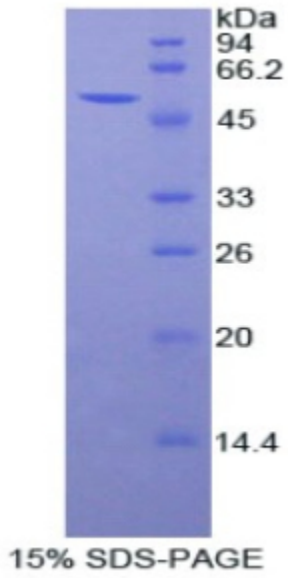
SDS-PAGE Image
