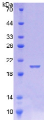
SDS-PAGE Image
