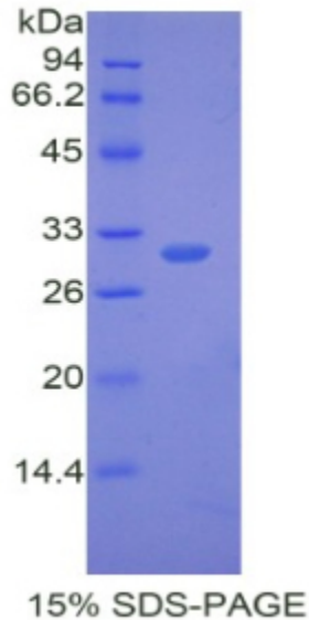
SDS-PAGE Image
