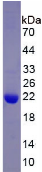
Figure. SDS-PAGE
