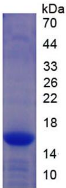
Figure. SDS-PAGE
