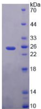
SDS-PAGE Image
