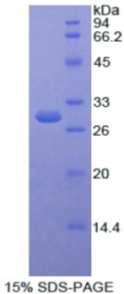
SDS-PAGE Image
