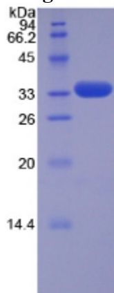
SDS-PAGE Image
