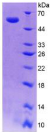
SDS-PAGE Image
