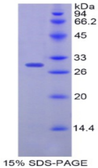
SDS-PAGE Image
