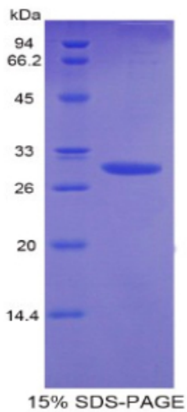
SDS-PAGE Image
