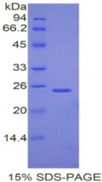
SDS-PAGE Image
