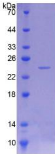
Figure. SDS-PAGE
