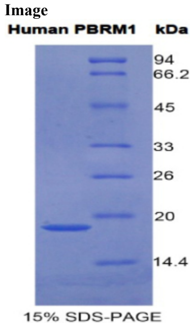
SDS-PAGE Image
