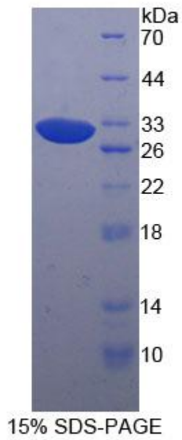
SDS-PAGE Image
