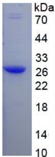
Figure. SDS-PAGE
