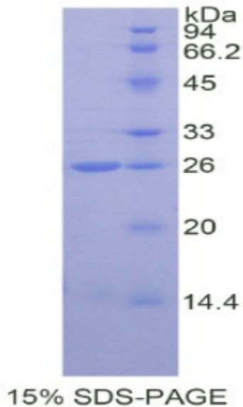
Figure. SDS-PAGE
