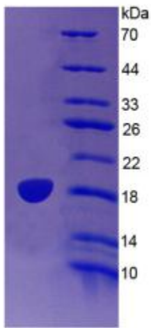
SDS-PAGE Image
