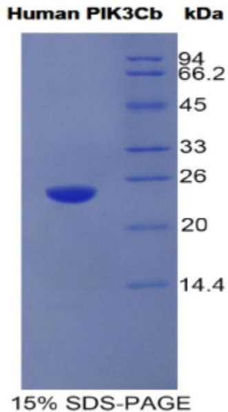
SDS-PAGE Image
