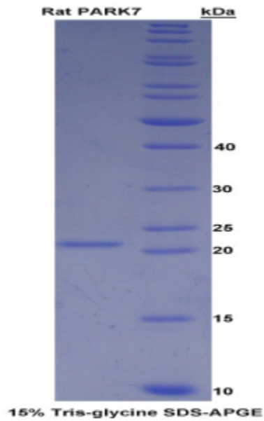
SDS-PAGE Image
