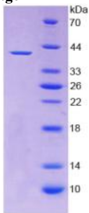
Figure. SDS-PAGE
