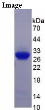
Figure. SDS-PAGE
