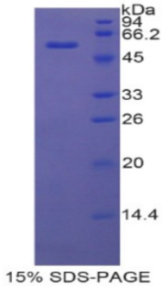
SDS-PAGE Image
