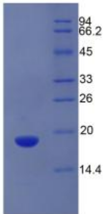
SDS-PAGE Image
